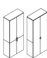
Libreria 2-4 ante/ Cabinet with 2-4 doors L 90 P 40 H 207
