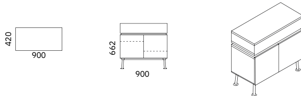
Azura middle cabinet
