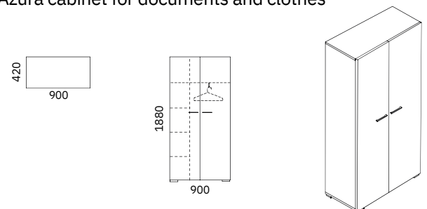
Azura cabinet for documents and clothes
