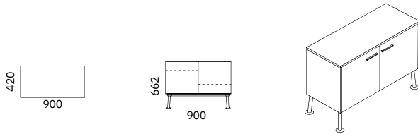
Azura low closed cabinet
