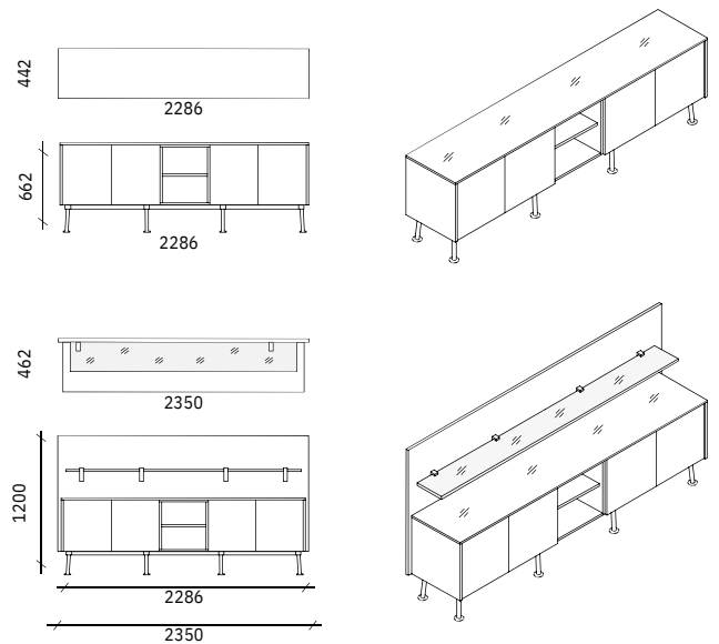
Azura wide executive showcase with open segment
