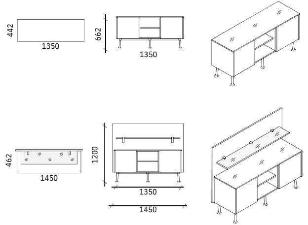
Azura narrow executive showcase with open segment
